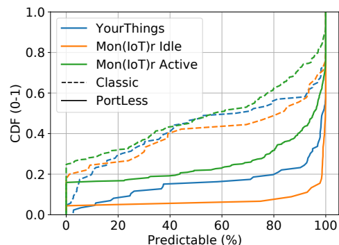
Figure 1: CDFs of the percentage of predictable traffic.
