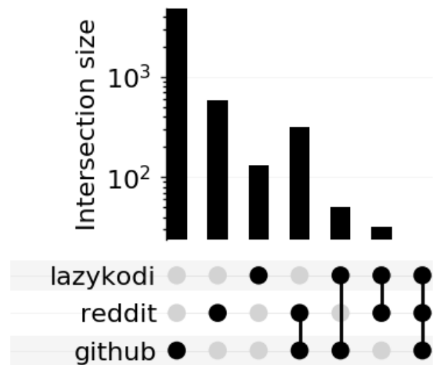
Figure 4: UpSet plot of addons directly found across search seeds. Each bar’s respective seeds are marked with a black dot.
