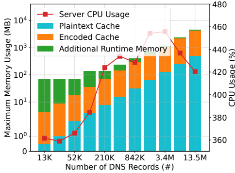
Figure 7: Memory and CPU as a function of cache size.
