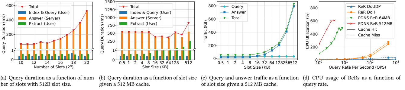
Figure 3: Benchmarking results for PDNS. Network latency is negligible.
