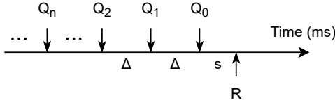
Figure 9: Illustration of the modeling for delayed response forwarding.
