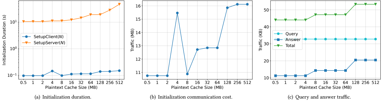
Figure 6: Additional benchmarking results. (a) Initialization duration, (b) communication cost during initialization, and (c) query and answer traffic as functions of the plaintext cache size.
