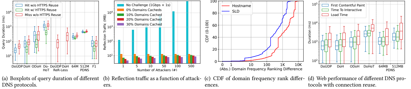
Figure 4: Evaluation of PDNS.
