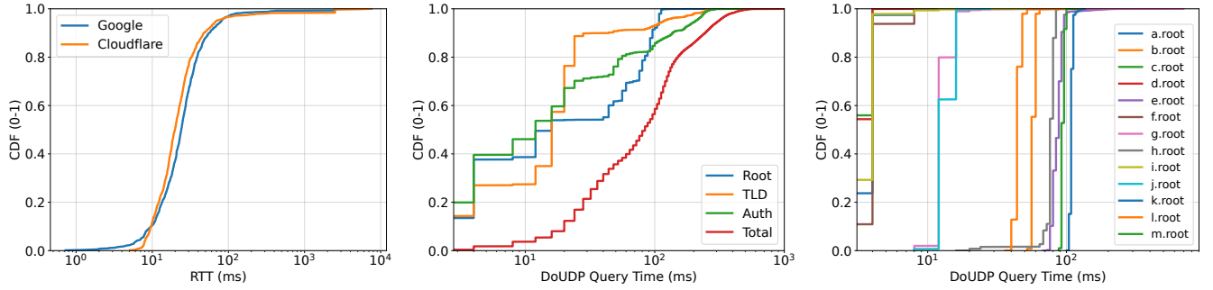
(a) CDF of RTT between 1,415 residential dVPN nodes and Google and Cloudflare DNS ReRs. (b) CDF of the duration of iterative DNS queries distinguishing between root, TLD, and final ANSes. (c) CDF of the duration of DoUDP queries per root ANS.
