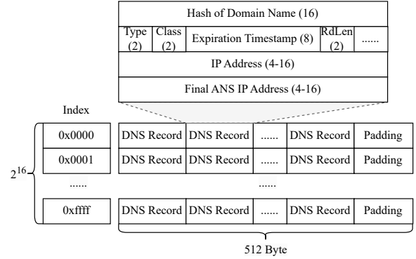
Figure 2: PDNS cache as a hash table with 2^{16} slots.
