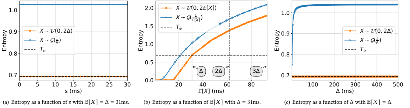
Figure 10: The effectiveness of delayed response forwarding to PDNS ReR.
